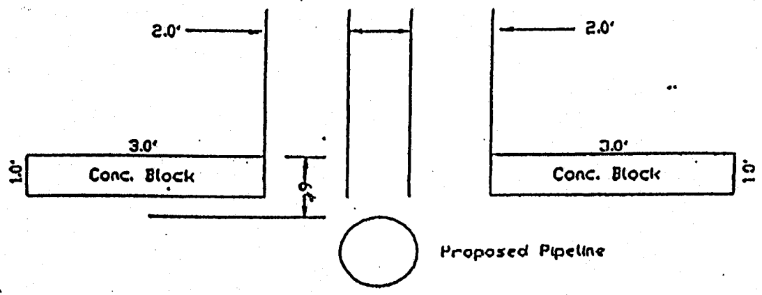
SECTION A - A' PIPELINE CROSSING HIGHWAY NOT TO SCALE
