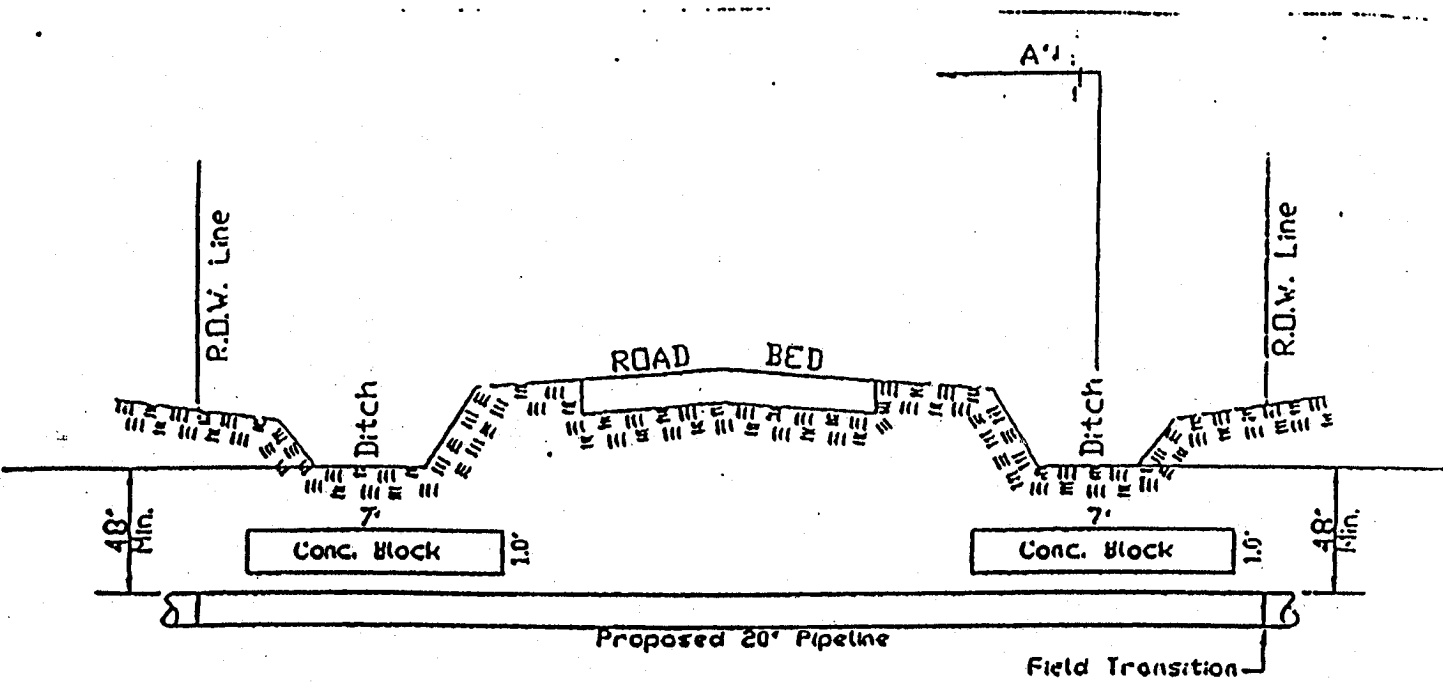
ELEVATION VIEW OF PIPELINE CROSSING HIGHWAY NOT TO SCALE
